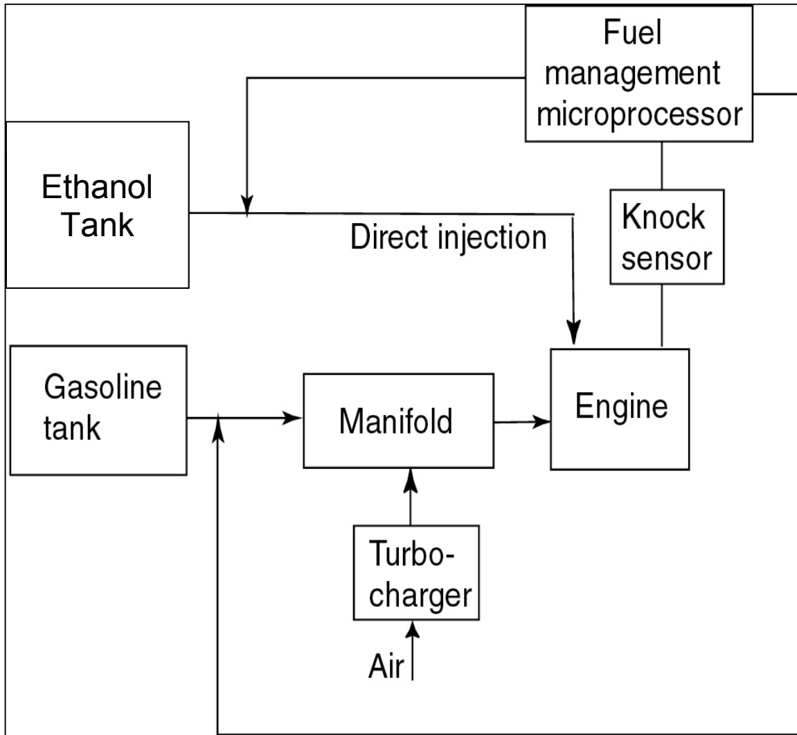
Figure 1. Fuel management system for “on-the-fly” direct injection of ethanol. A knock sensor would be used to determine when ethanol is needed and how much should be used.
